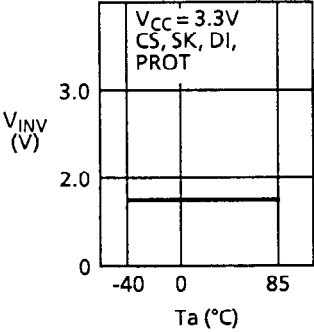
1.25 Input inversion voltage V_{INV} – Ambient temperature T_a
